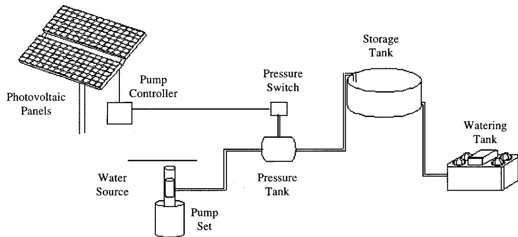
Figure 3. Direct-coupled solar pumping system.
