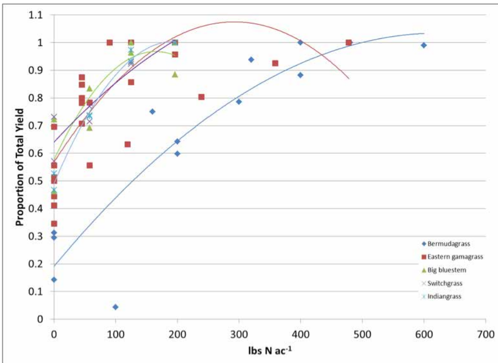
Fig. 10. Yield response to nitrogen (N) fertilization for bermudagrass, eastern gamagrass, big bluestem, switchgrass, and indiangrass. Yield (vertical axis) is not expressed in the quantity of hay produced, but rather as a proportion of each species' total yield potential. The native grasses start (0 units N) at about 50-60% of their yield potential and reach their peak at about 100 units N. Eastern gamagrass peaks at about 300 units N per acre. This is in contrast with bermudagrass which starts at only 20% of its yield potential at 0 units N.
