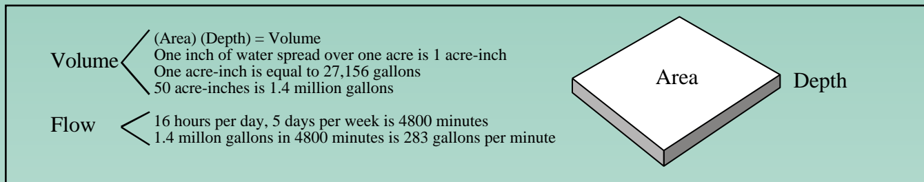
Figure 2. The depth of water applied over an area gives the volume of water required and the flowrate of the pump required to supply this volume in a given amount of time.
