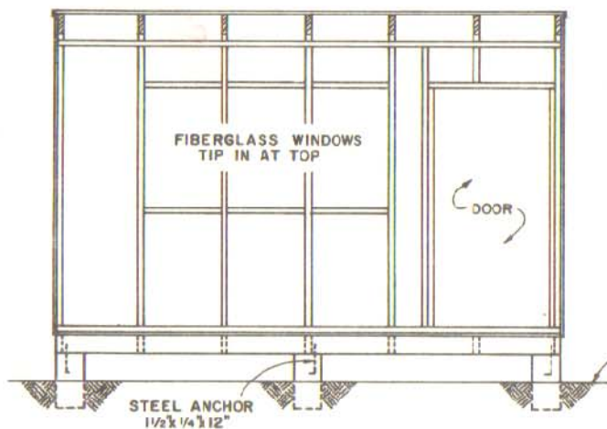
FRONT ELEVATION FRAMING
